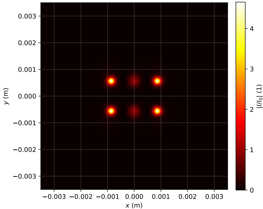
Intensity profile I(x, y, z = 0.796)/I_0 , P_{in}=5.0P_{cr} , artificial time
